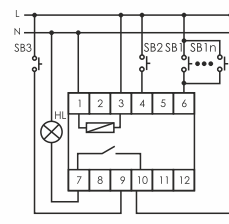
BIS-412i (LED)
