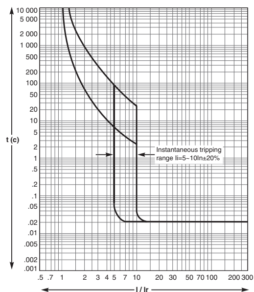
BA-335A (500-630 A)
