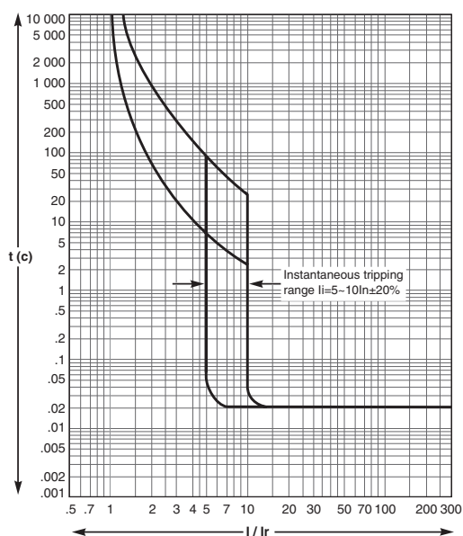
BA-335A (250-400 A)
