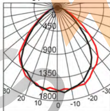
Alumogips-20/ice 295x595
