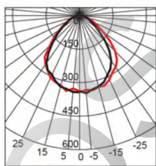
ЛПО 2x36-CSVT/ICE-R
