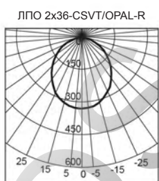
ЛПО 2x36-CSVT/OPAL-R
