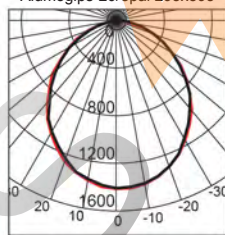
Alumogips-20/opal 295x595
