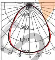
CSVT Operlux-30/prisma/R-2
