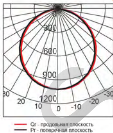
LED-PL-CSVT-36 595x595
