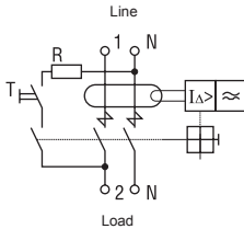
Figure 3. Electric schematic diagram of 2-polar VD
