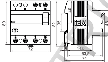
Figure 2. Overall and installation dimensions of 4-polar VD
