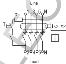
Figure 4. Electric schematic diagram of 4-polar VD
