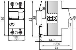
Figure 1. Overall and installation dimensions of 2-polar VDs
