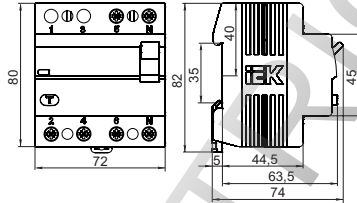
Figure 2. Overall and installation dimensions of 4-polar VDs
